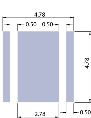
Recommended PCB Footprint
