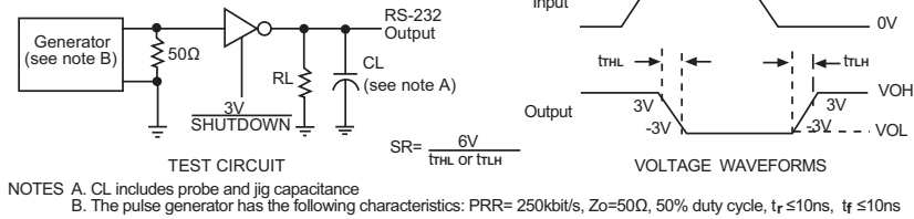
Figure 1. Driver Slew Rate
