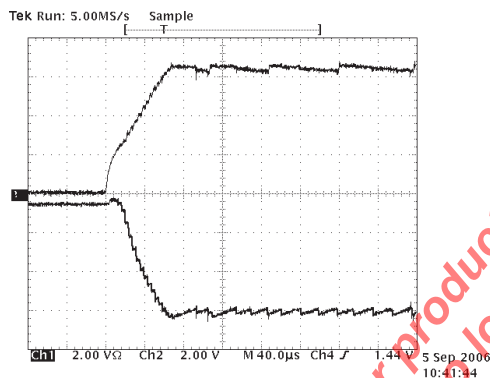
SP3225E/SP3227E Charge Pump Power On Time, V_{cc}=3.3V
