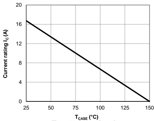
Figure 11: Current De-rating
