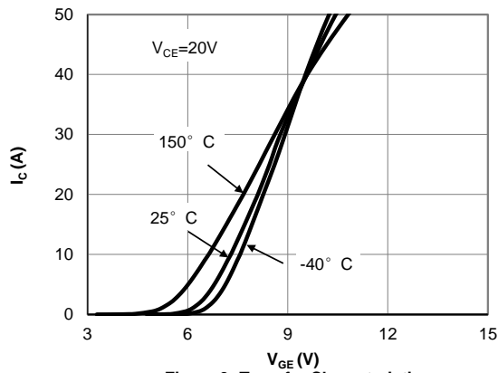
Figure 3: Transfer Characteristic
