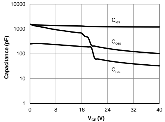
Figure 8: Capacitance Characteristic
