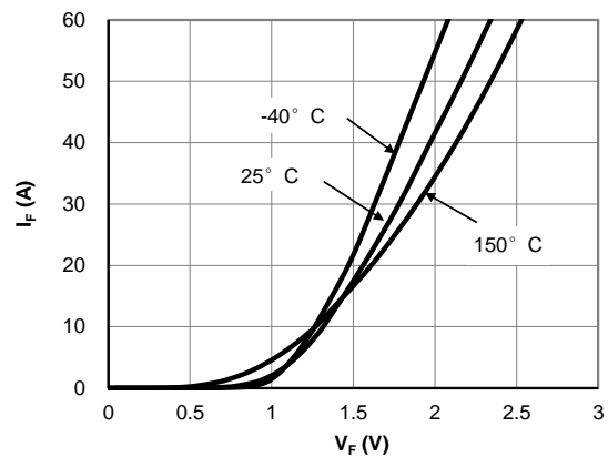
Figure 4: Diode Characteristic
